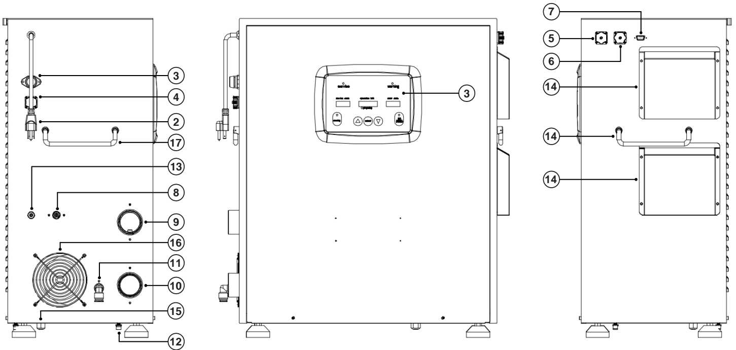
Figure 1. OWS-1 Dimension Drawing Showing Connections
